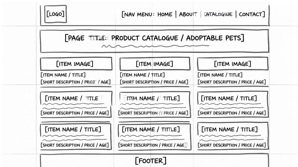
Figure 2 Products Wireframe
